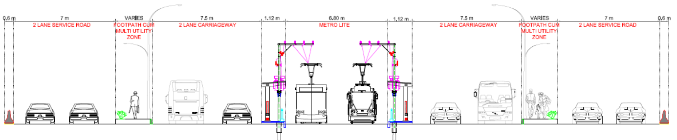
TYPICAL CROSS SECTION - METRO LITE
